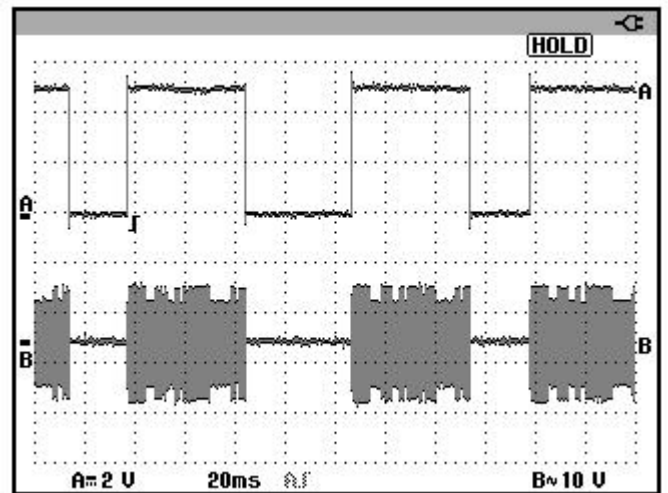
A pure data signal
