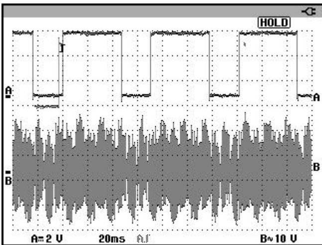
Noise Induced from line side AC
